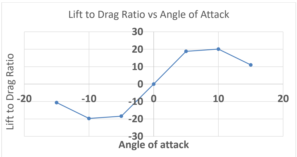
Fig. 7. Lift to Drag Ratio vs Angle of Attack
