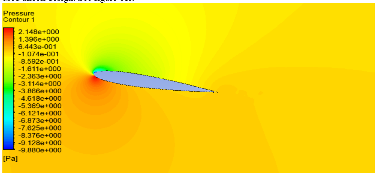
Fig. 8. Pressure Contour NACA 0012 (10° AOA)
