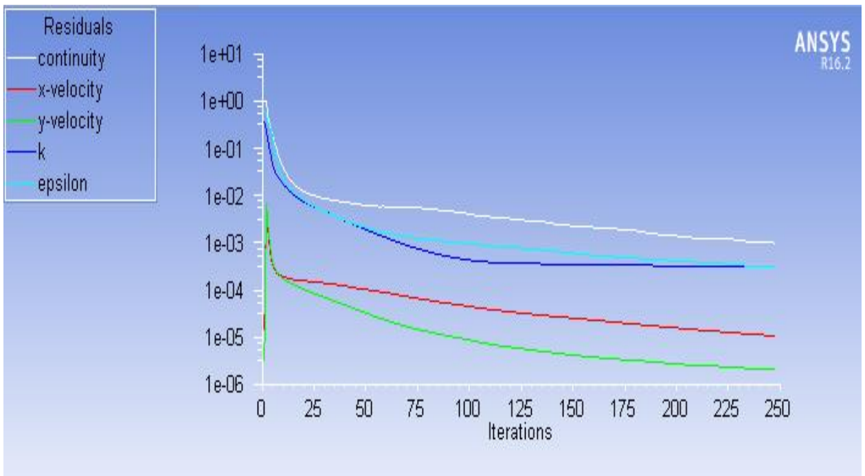
Fig. 4. Residual Convergence NACA0012
