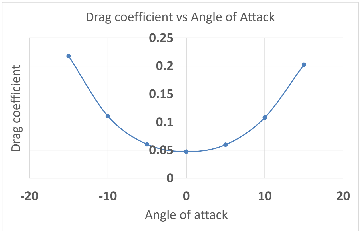
Fig. 6. Drag Coefficient vs Angle of Attack
