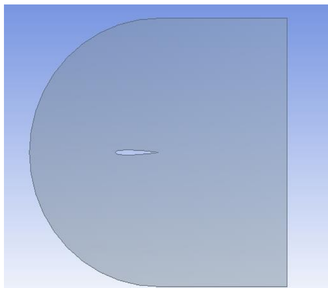
Fig. 2. C-Type Geometry NACA0012
