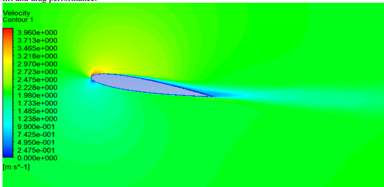
Fig. 10. Velocity Contour NACA 0012 (10° AOA)
