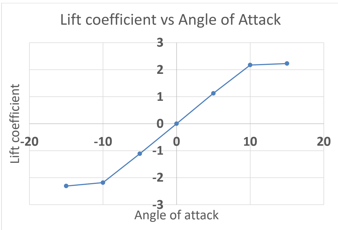
Fig 5: Lift Coefficient vs Angle of Attack
