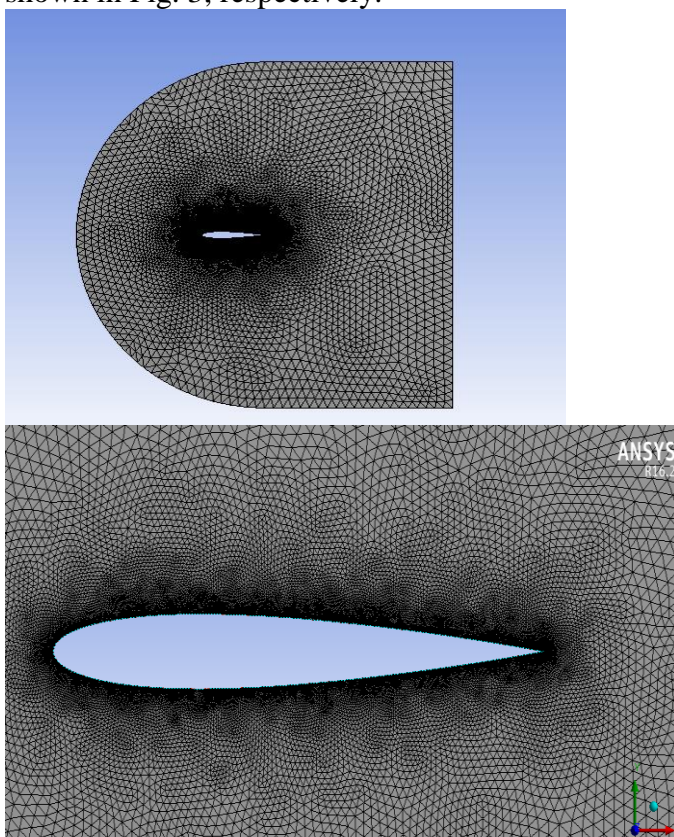
Fig. 3. (a) Mesh around NACA0012 airfoil (b) Mesh details close to airfoil.
